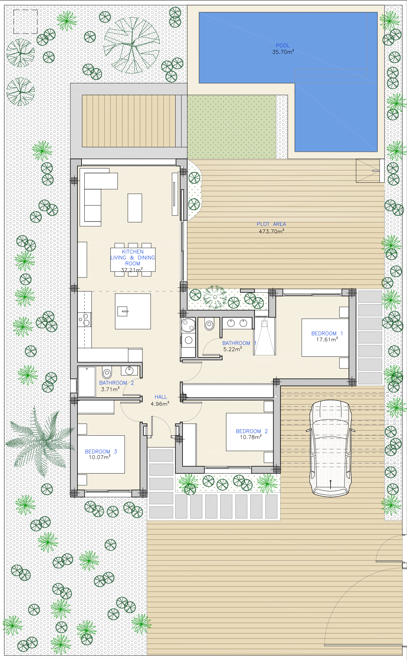
GROUND FLOOR
